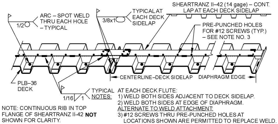
FIGURE 7-DETAILS FOR SHEARTRANZ® II-42 FOR PLB™-36 &amp; SHEARTRANZ® II FOR HSB®-36 DECK
